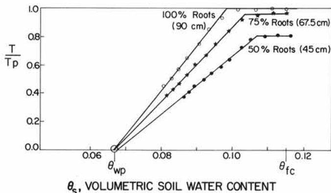
Fig. 3. Ratio of transpiration to potential transpiration ( T/TP ) as a function of volumetric soil water content ( \theta ) of a sandy soil for three simulated root length densities at a common leaf area index. \theta_{fc} and \theta_{wp} are the soil water contents at field capacity and at the permanent wilting point, respectively.
