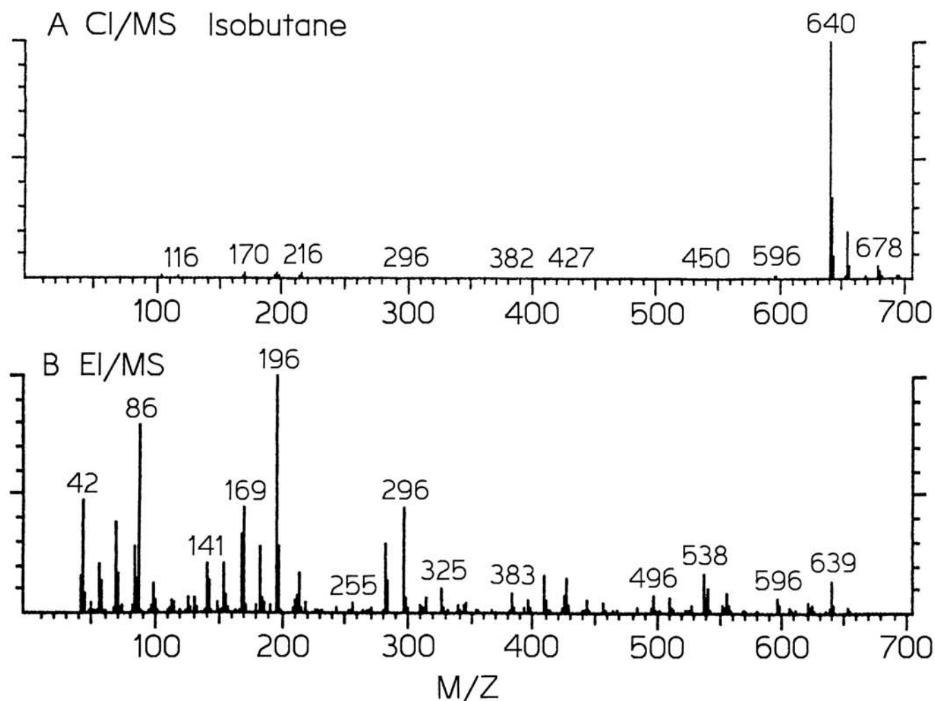
Fig. 2. Mass spectra of crystalline enniatin isolated from corn medium fermented by Fusarium tricinctum NRRL 26430. A , Isobutane chemical ionization spectrum and B , 70 V electron impact spectrum.
