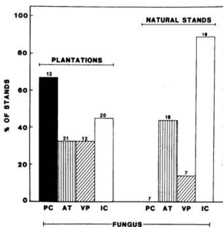
Fig. 2. Percentage of sand pine stands from which various known and/or suspected root-pathogenic fungi were isolated in Florida. PC = Phytophthora cinnamomi , AT = Armillariella tabescens , VP = Verticilladiella procera , IC = Inonotus circinatus . Numbers of stands on which percentages are based are noted at the top of each bar.
