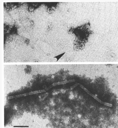
Fig. 4. Isometric and rigid rod viruslike particles as seen under the electron microscope in (top) a single cleistothecium extract and (bottom) partially purified leaf tissue (50 g) bearing cleistothecia. The grid was stained with 1% uranyl acetate. Bar = 100 nm.
