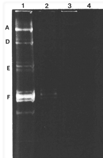
Fig. 3. Electrophoretic analysis in a 6% polyacrylamide gel of dsRNA extracted from 1) pure cleistothecia from Rosette, 2) pure cleistothecia from Colobel-256, 3) Colobel-256 leaves cleaned of cleistothecia, and 4) Rosette leaves cleaned of cleistothecia. Each cleistothecia sample was collected from 30 g of leaf tissue and each leaf sample consisted of 15 g. Both leaf samples were included as controls. Samples were analyzed by electrophoresis in 6% polyacrylamide gel for 11 hr at 20 mA, and the gel was stained in ethidium bromide.
