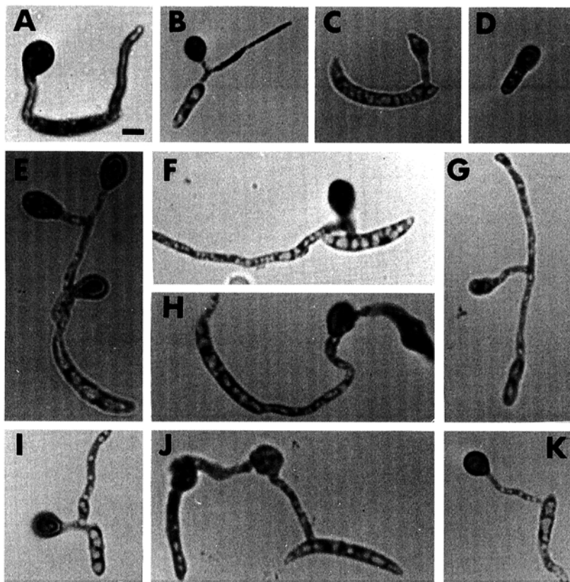
Fig. 4. Appressorial formation of Colletotrichum capsici and C. gloeosporioides in association with different compounds. (A) C. capsici in \text{CaCl}_2 at 10^{-3} M; (B) C. gloeosporioides in \text{CaCl}_2 at 10^{-3} M; (C) C. capsici in \text{AlCl}_3 at 10^{-3} M; (D) C. gloeosporioides in \text{AlCl}_3 at 10^{-3} M; (E) C. capsici in sucrose at 10^{-3} M; (F) C. capsici in 1 \mu\text{g} a.i. per ml of isoprothiolane; (G) C. gloeosporioides in \mu\text{g} a.i. per ml of tricyclazole; (H) C. capsici in 1 \mu\text{g} a.i. per ml of fthalide; (I) C. gloeosporioides in 1 \mu\text{g} a.i. per ml of fthalide; (J) C. capsici in 1 \mu\text{g} a.i. per ml of tricyclazole; (K) C. gloeosporioides in \mu\text{g} a.i. per ml of isoprothiolane. Bar in (A) is ca 7 \mu\text{m} for all figures.
