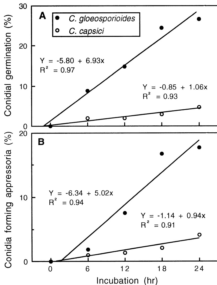
Fig. 1. Conidial germination and appressorial formation of Colletotrichum capsici and C. gloeosporioides on glass slides at different incubation periods.
