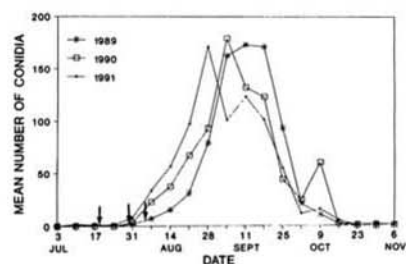
Fig. 3. The mean weekly number of conidia counted during 1989, 1990, and 1991 seasons and times the first disease symptoms were observed (i).
